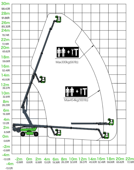
LT26JE Working Range
